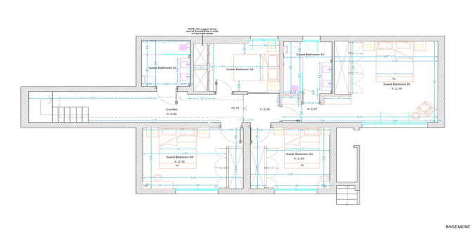
BASEMENT
