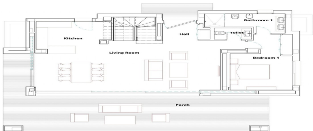
IROKO 4 - BAR GROUND FLOOR
