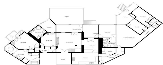
MAIN FLOOR
